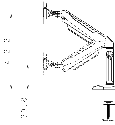
HEIGHT ADJUSTMENT VIEW
