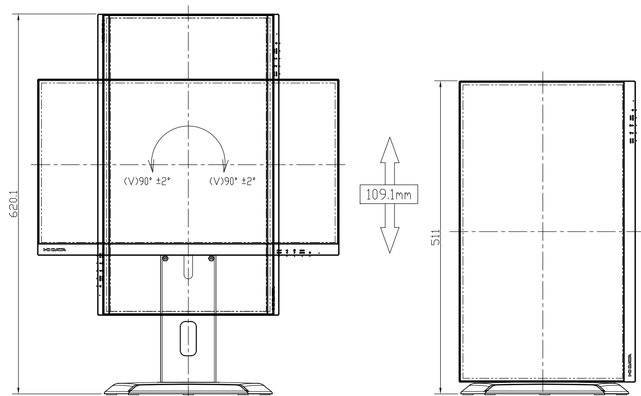
PIVOT VIEW
