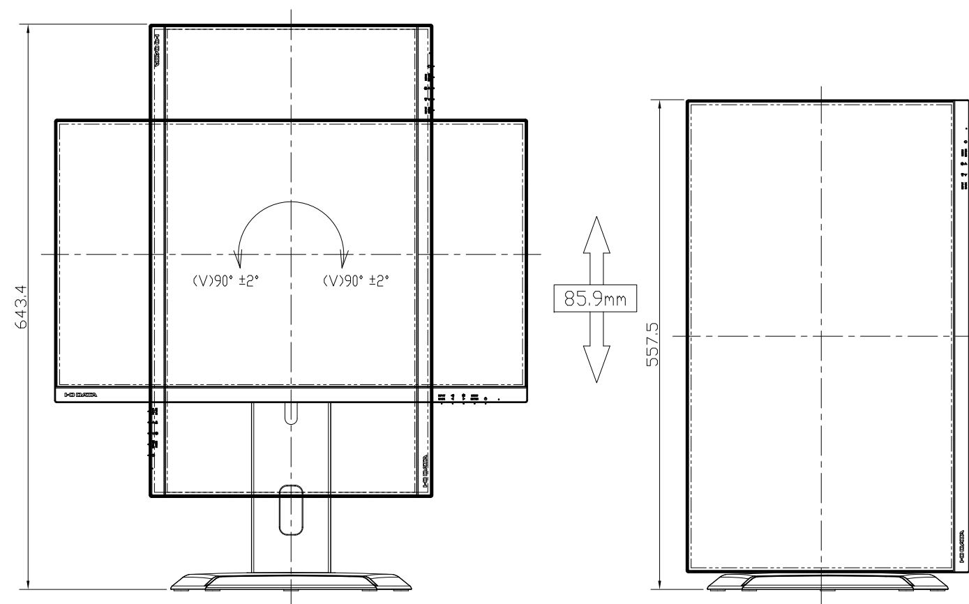
PIVOT VIEW
