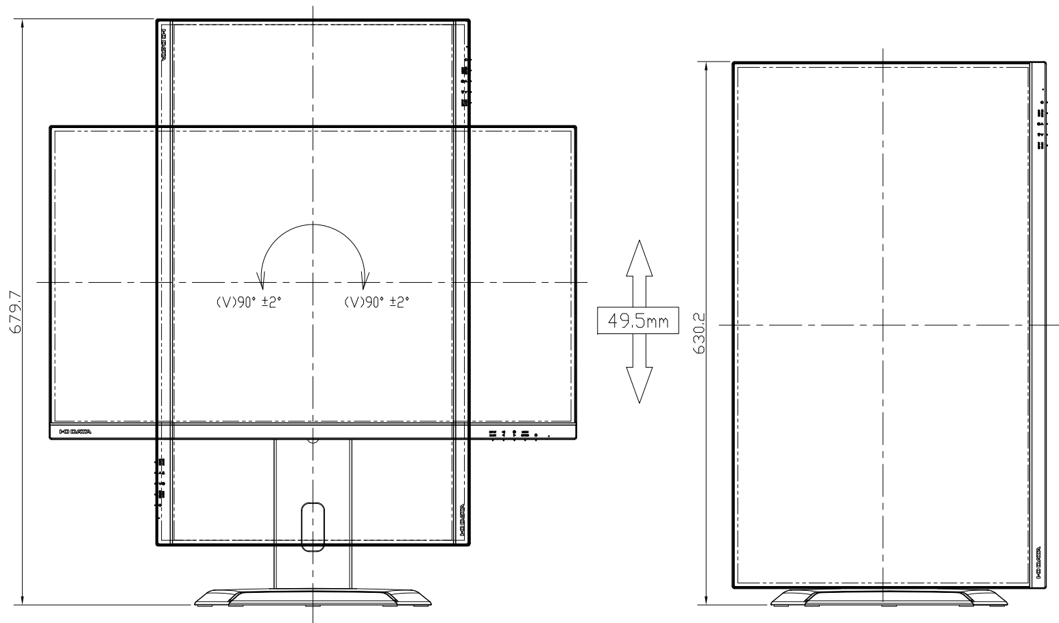
PIVOT VIEW
