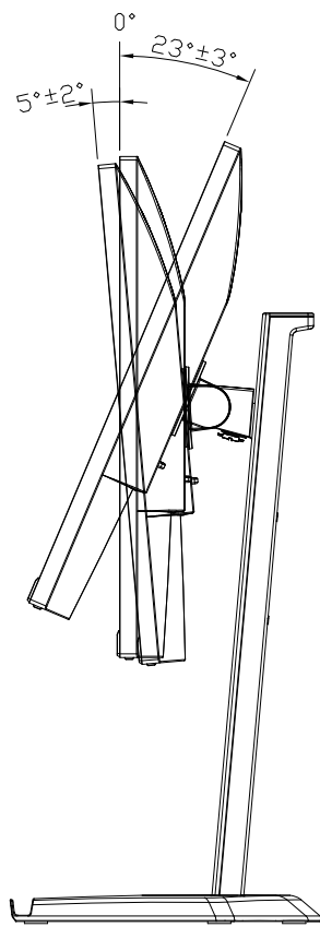
TILT VIEW
