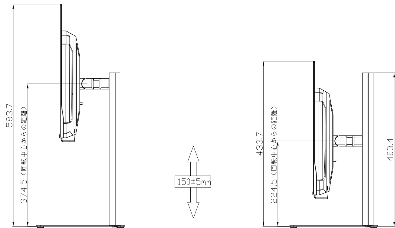
HEIGHT ADJUSTMENT VIEW
