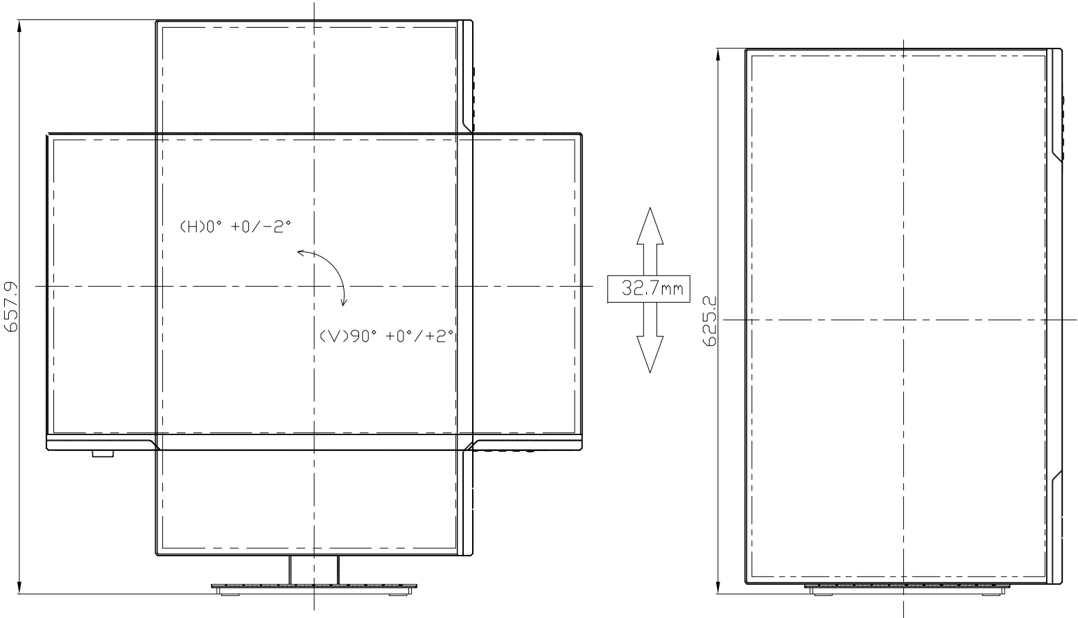
PIVOT VIEW
