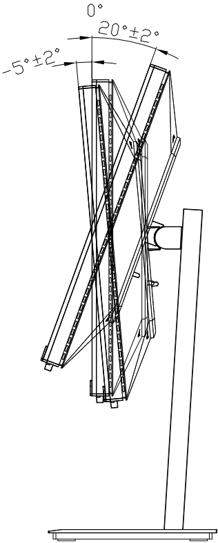
TILT VIEW
