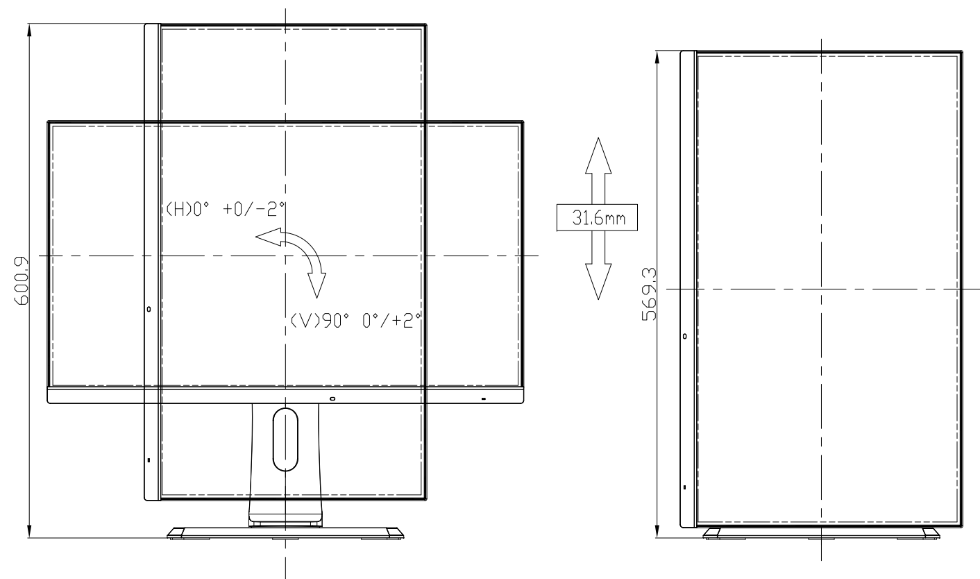
PIVOT VIEW
