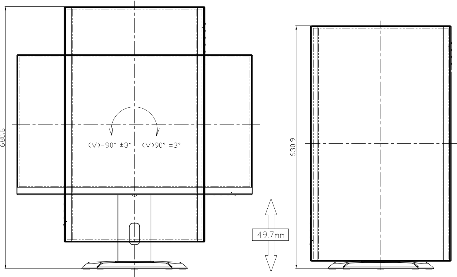
PIVOT VIEW
