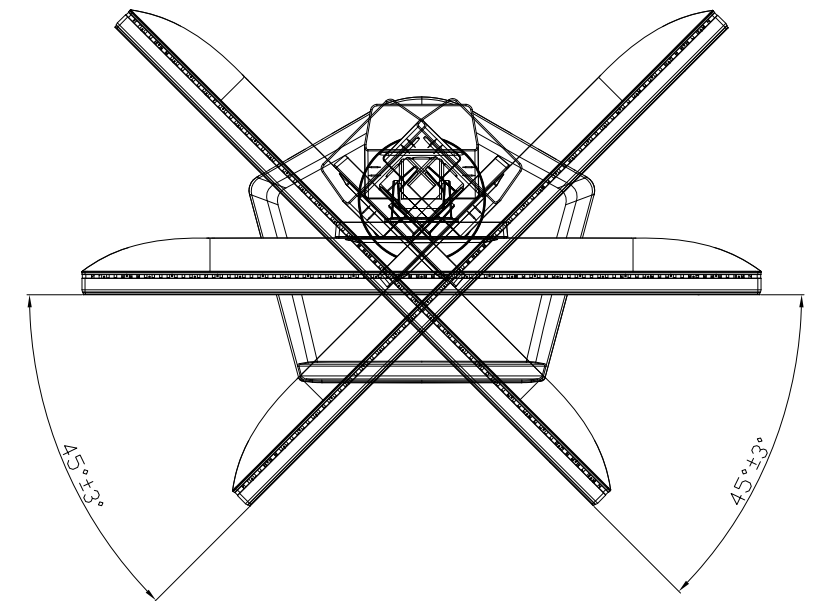
SWIVEL VIEW
