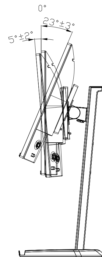
TILT VIEW
