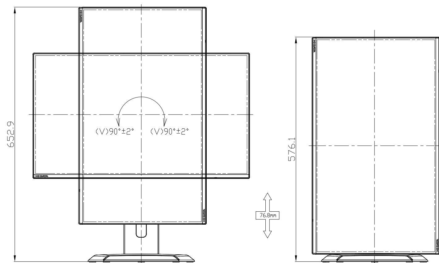
PIVOT VIEW
