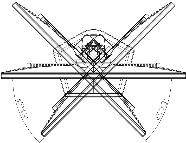
SWIVEL VIEW
