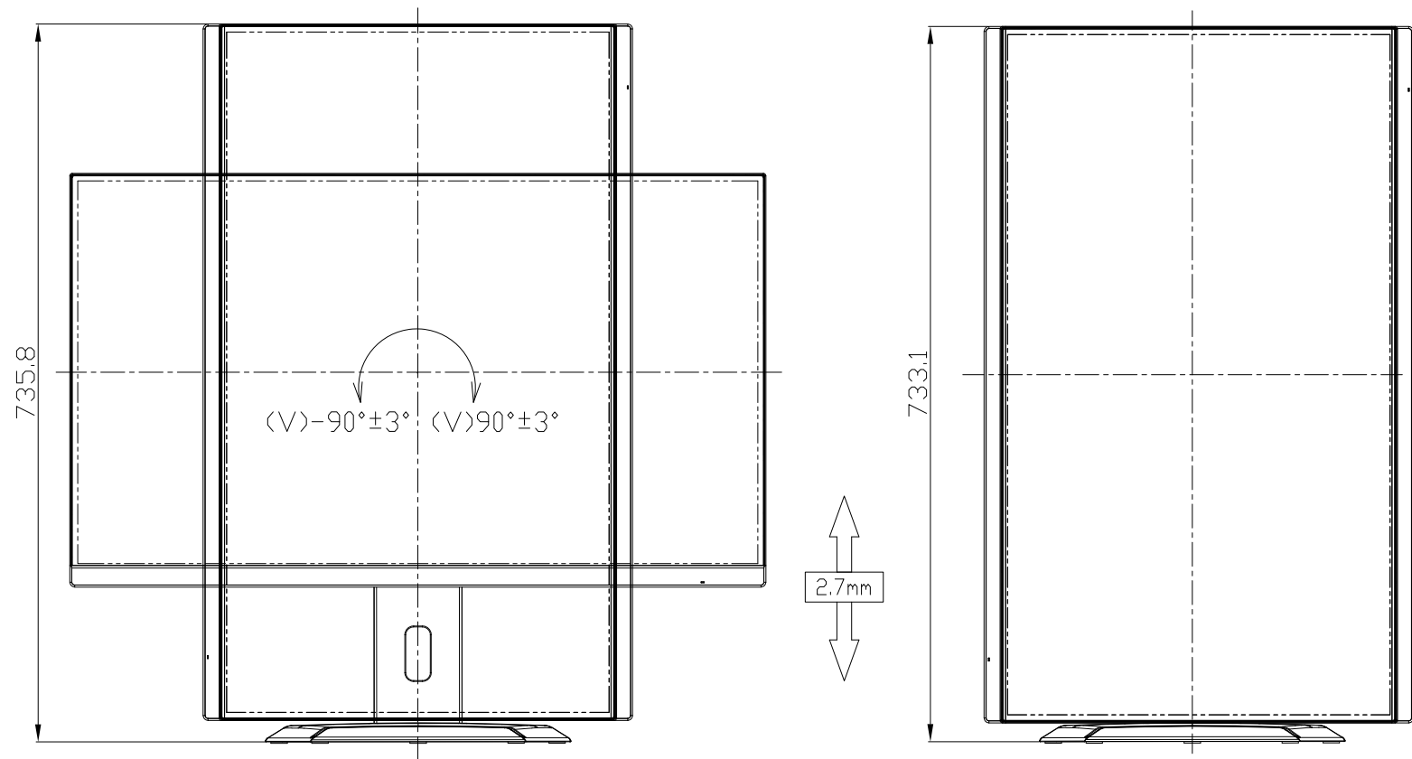
PIVOT VIEW
