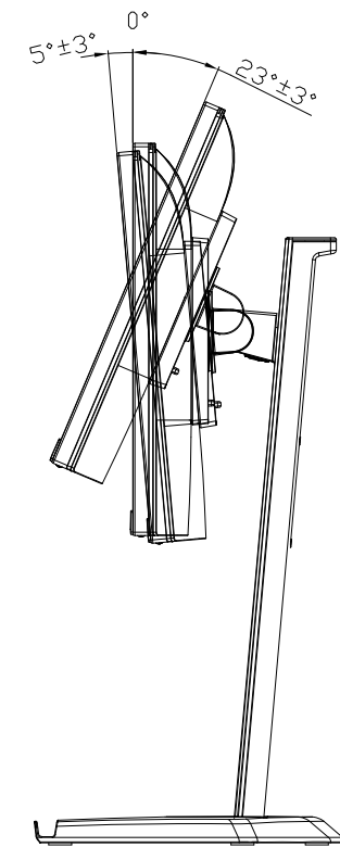
TILT VIEW
