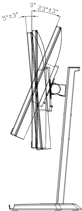
TILT VIEW
