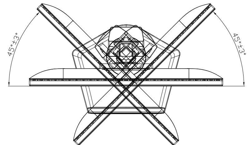
SWIVEL VIEW
