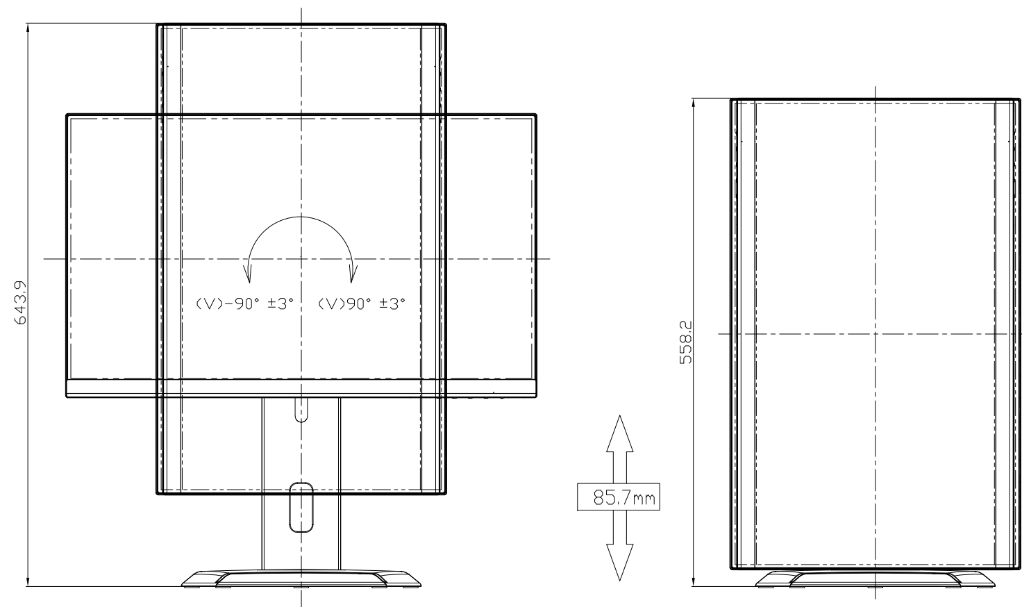
PIVOT VIEW
