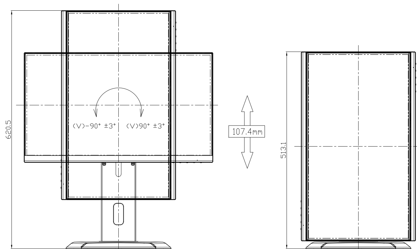
PIVOT VIEW
