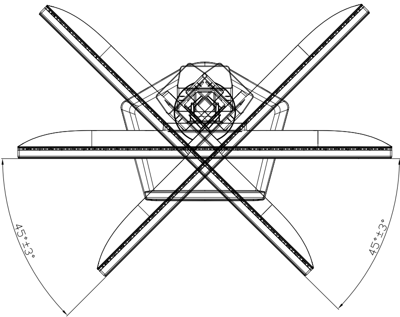
SWIVEL VIEW
