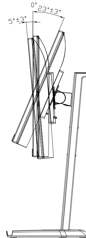
TILT VIEW
