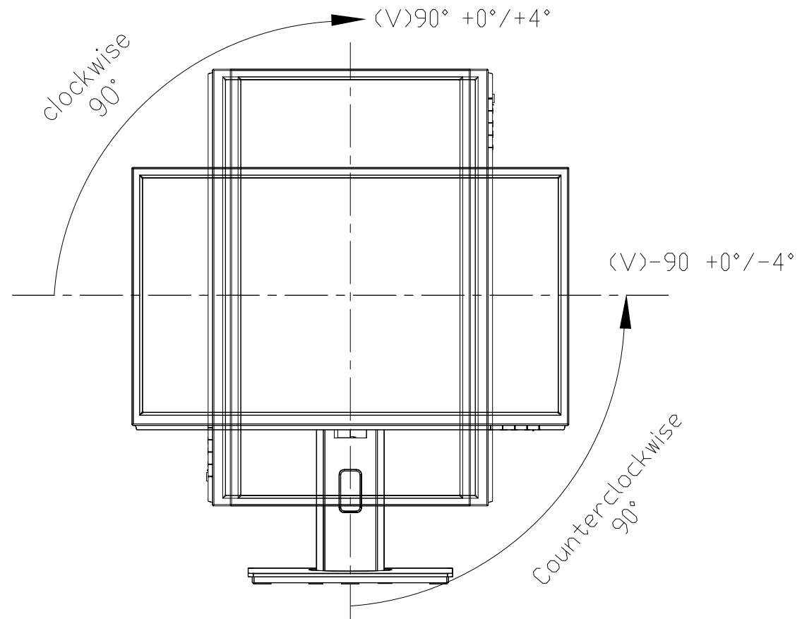
Pivot view
