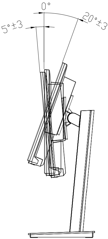
TILT VIEW
