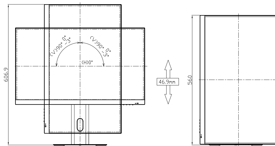
PIVOT VIEW
