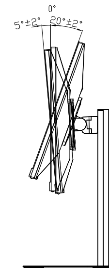
TILT VIEW
