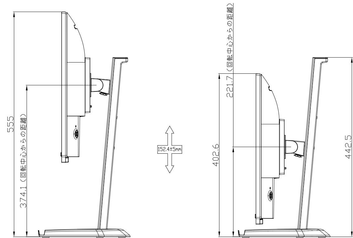
HEIGHT ADJUSTMENT VIEW
