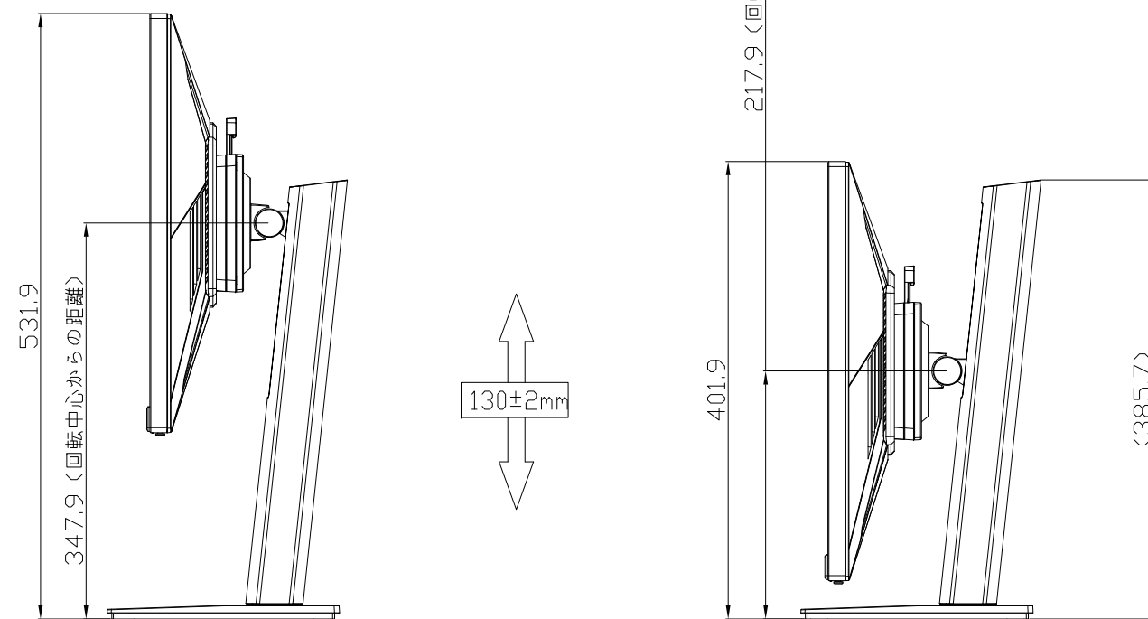
HEIGHT ADJUSTMENT VIEW
