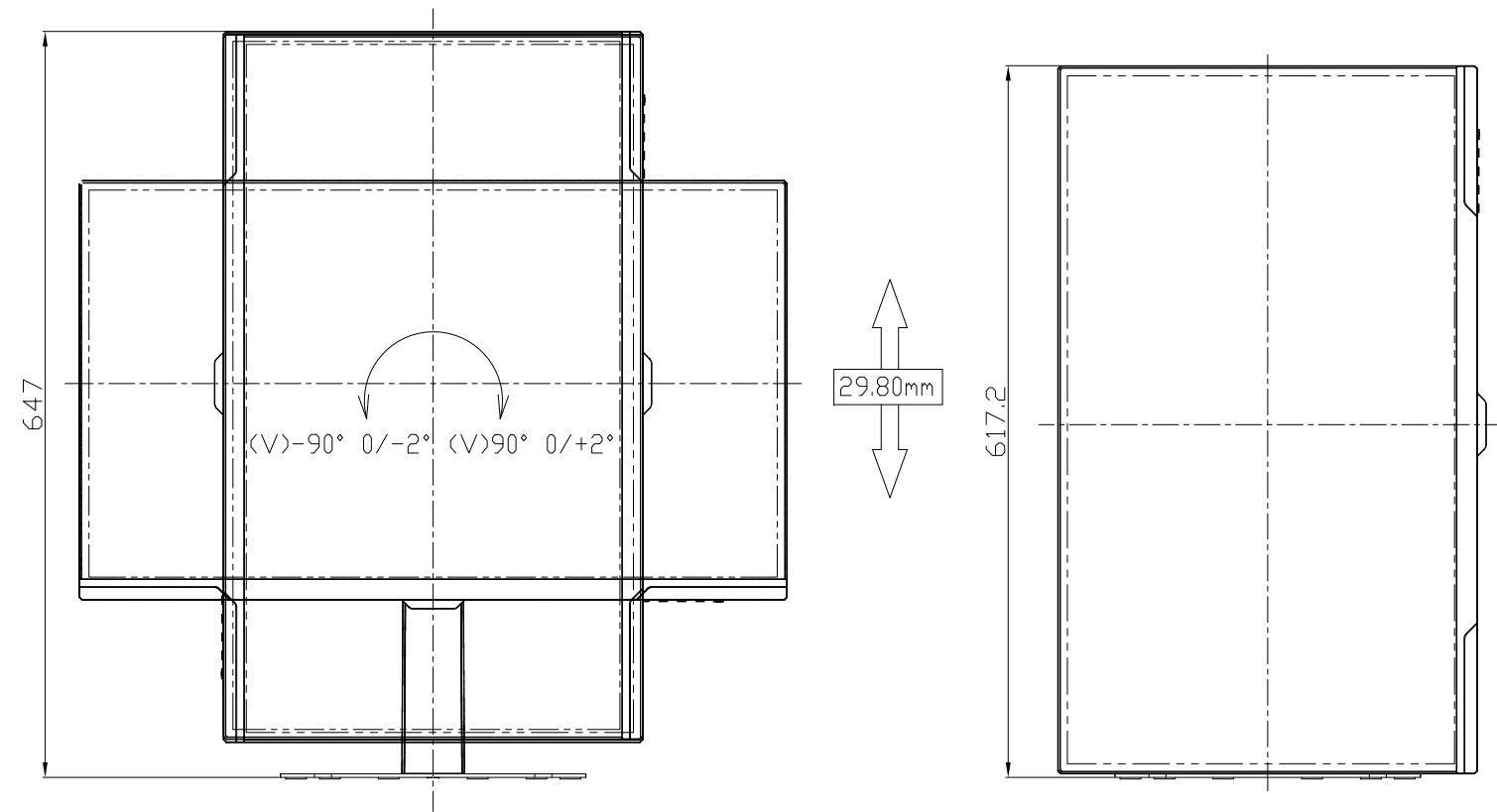
PIVOT VIEW
