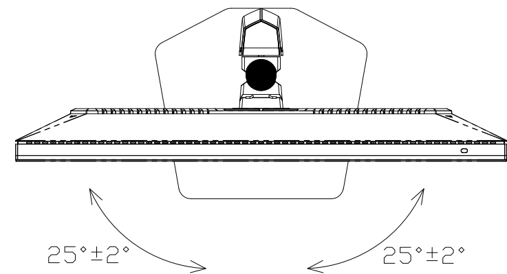
SWIVEL VIEW
