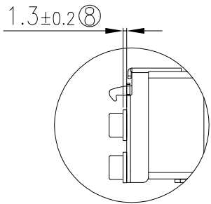
DETAIL-A SCALE 3:1
