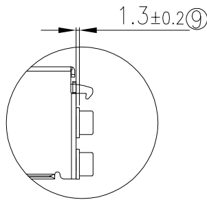
DETAIL-B SCALE 3:1
