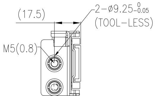
DETAIL-A SCALE 3:1
